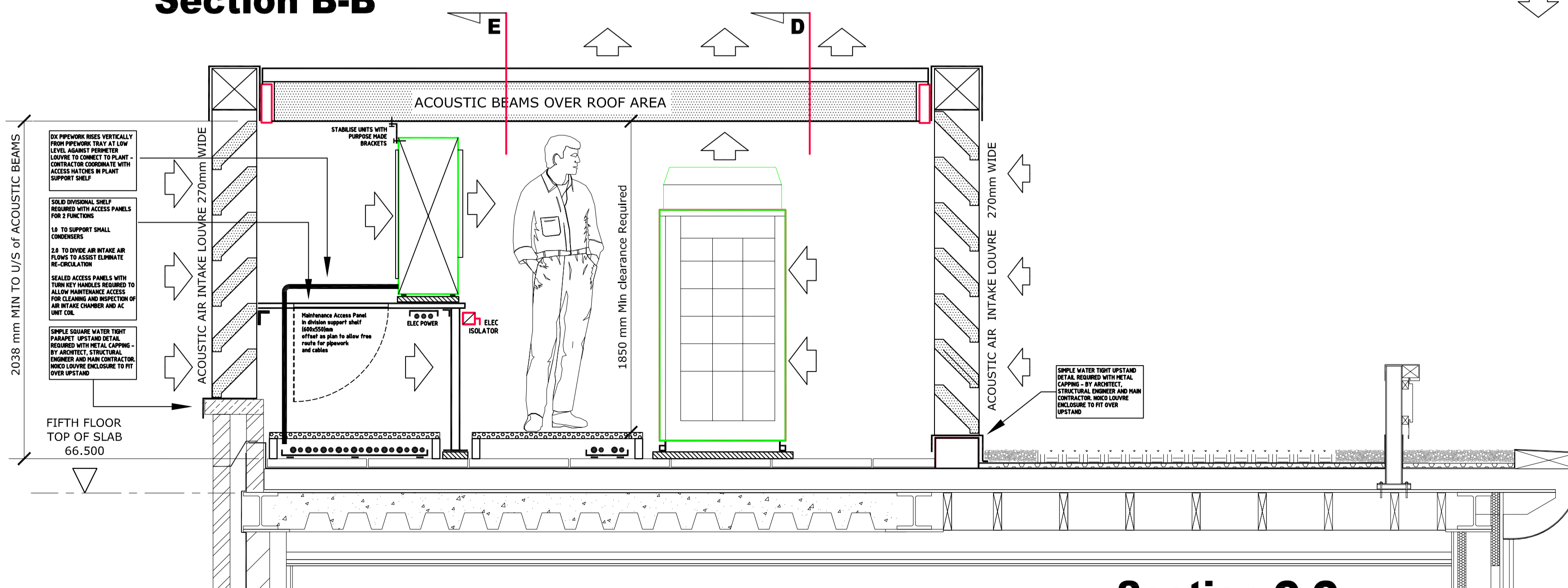
Section C-C
